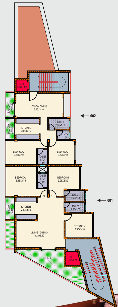
UPPER GROUND FLOOR PLAN
